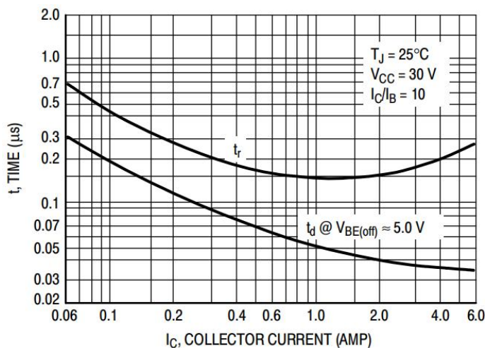
Figure 3. Turn-On Time
