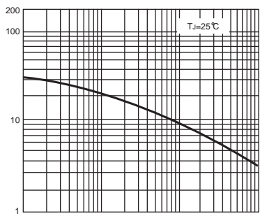
FIG. 5-TYPICAL JUNCTION CAPACITANCE
