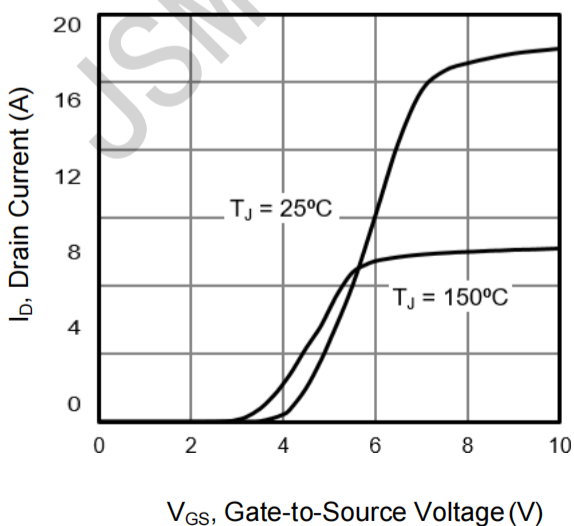
Figure 5. Transfer Characteristics
