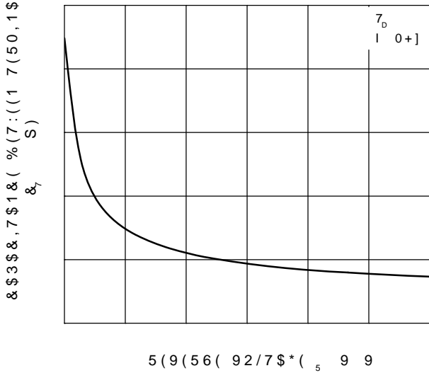
Dynamic Resistance vs. Forward Current
