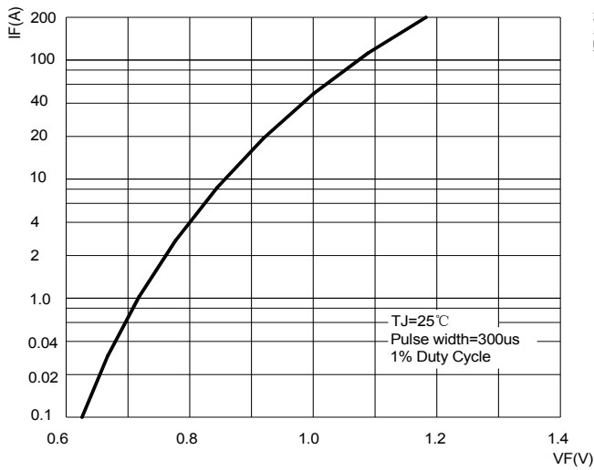
FIG.3: Forward Voltage
