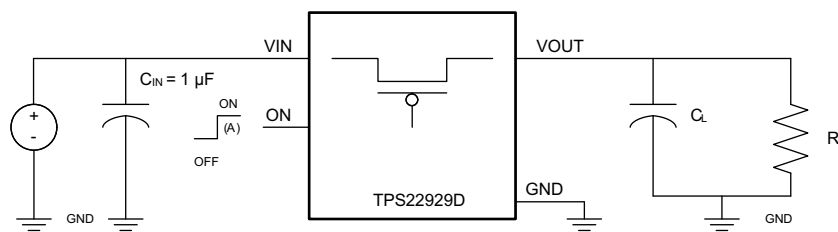
Figure 20. Test Circuit
