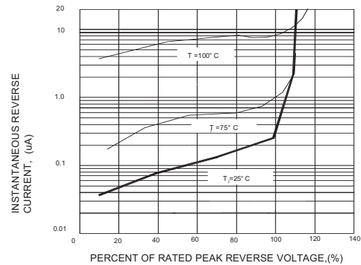
FIG.4-TYPICAL REVERSE CHARACTERISTICS
