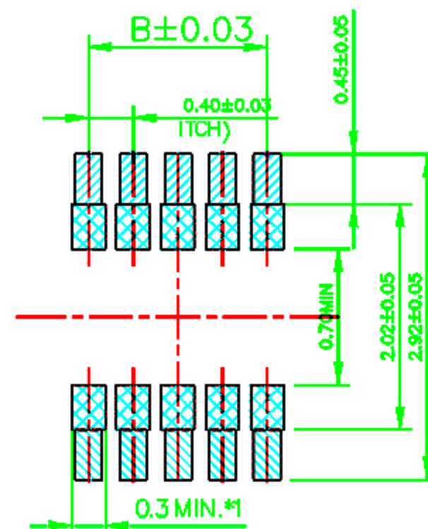
RECOMMENDED PCB LAYOUT TOP VIEW (TOL:±0.05)
